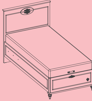
BAZALI KARYOLA (100x200cm) G:107 Y:118 D:211 cm 20.21.1707.00
