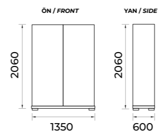
GARDROP / WARDROBE
