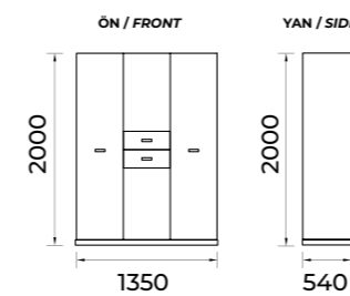
GARDROP / WARDROBE
