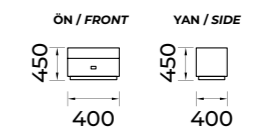
KOMODİN / COMMODE
