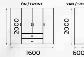
4 KAPAKLI GARDROP 4-DOOR WARDROBE
