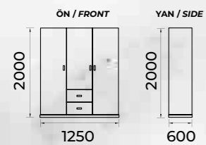
3 KAPAKLI GARDROP 3-DOOR WARDROBE
