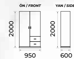
2 KAPAKLI GARDROP 2-DOOR WARDROBE
